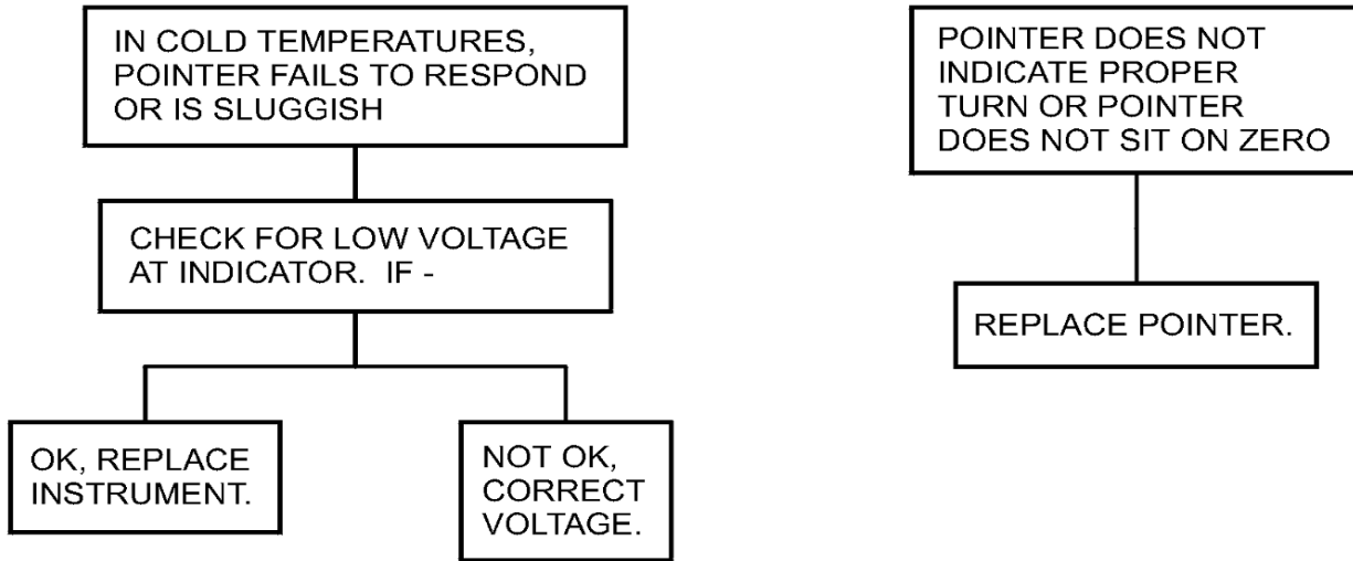
Figure 101 : Sheet 3 : Turn and Bank Indicator Troubleshooting Chart
