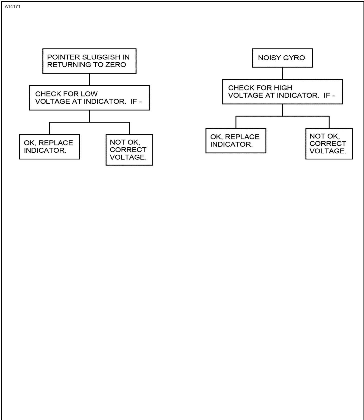
Figure 101 : Sheet 2 : Turn and Bank Indicator Troubleshooting Chart
