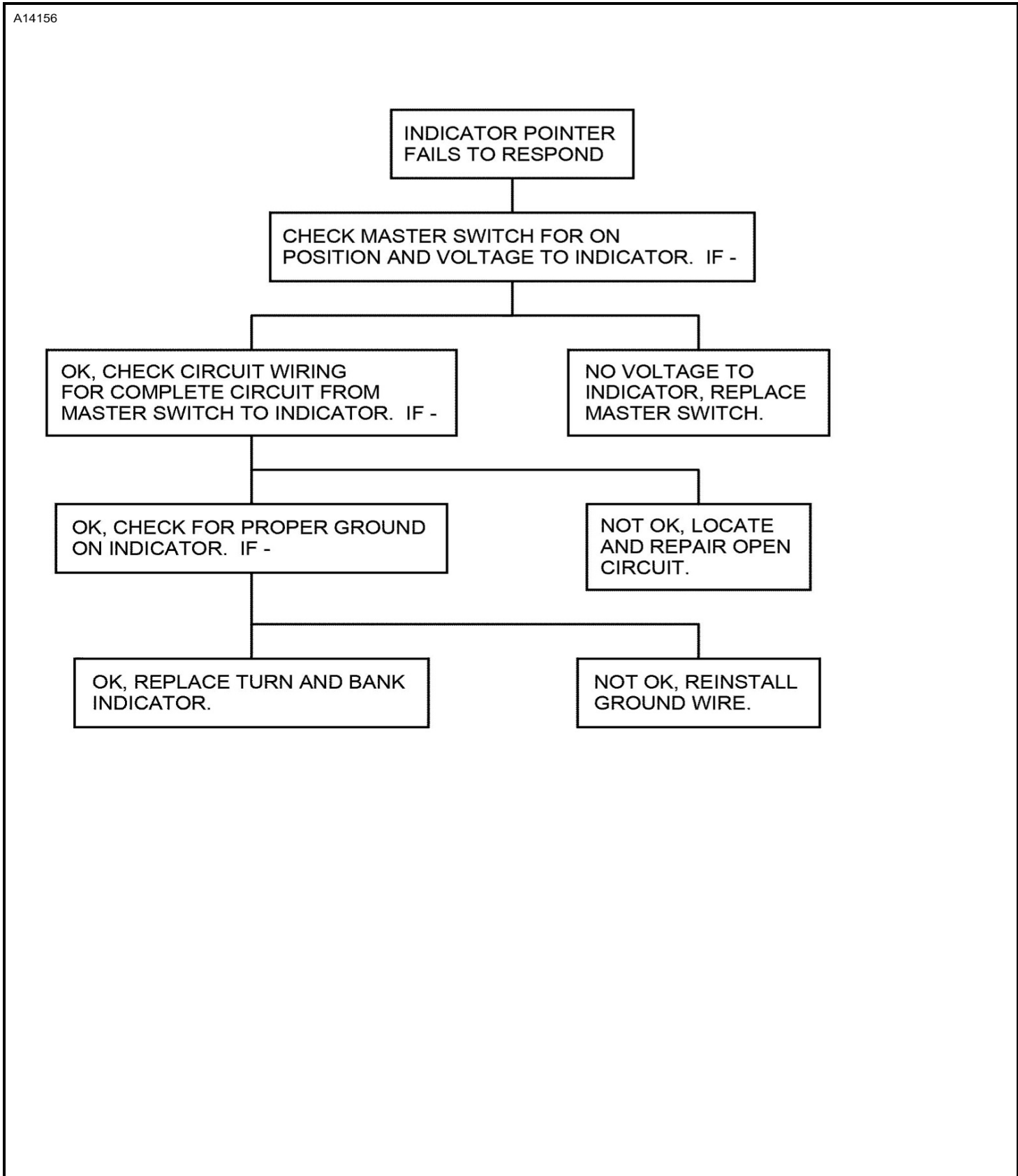
Figure 101 : Sheet 1 : Turn and Bank Indicator Troubleshooting Chart
